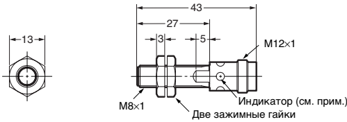
E2A-S08KS02-M1-□□
