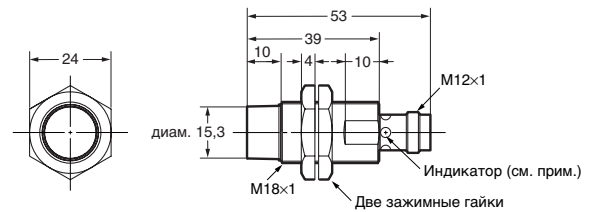
E2A-M18KN16-M1-□□/E2A-S18KN16-M1-□
