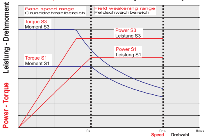
Power and torque characteristic
