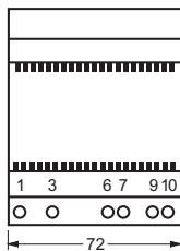
4AC2 962-4 4AC2 964-0
