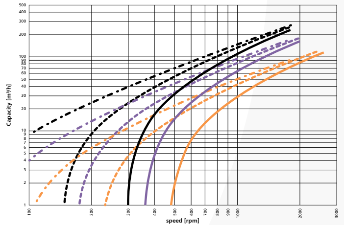
Performance Curve - 6 bar
