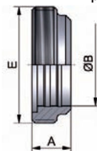
DS expanding male part
