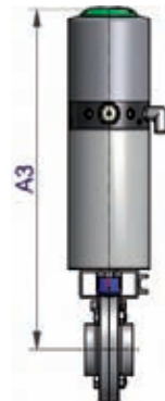
butterfly valve SV04 actuator PAMS-size 1/2 NC + TOP Art.-Nr. 5xxxx-xxxxx60
